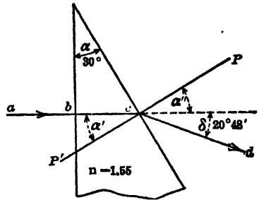
Refraction of Light through a Prism Method of Perpendicular Incidence
